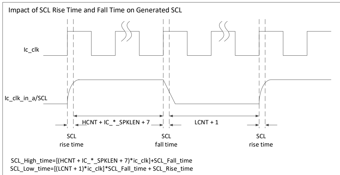
Figure 89 Rising and Falling Time Parameter Configuration Diagram
